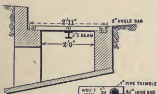
FIG. 1. FLUSHTANK
